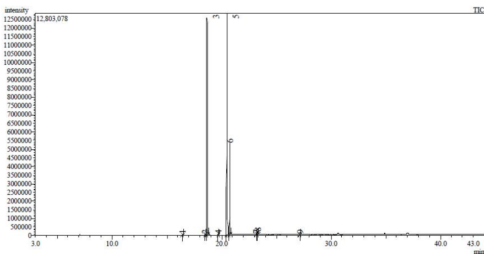
Fig.2. Chromatogram of fatty acid methyl esters from Telfairiapedata seed kernel crude oil analyzed by gas chromatography (GC)
