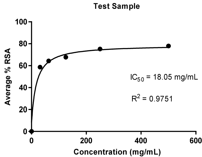
Fig.4. Nonlinear regression curve showing the IC 50 value of crude oil from the seed kernels of Telfairiapedata
